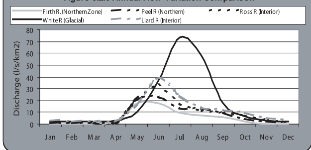
Figure 3.2.3 Annual Flow Variation Comparison
