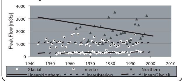
Figure 3.2.2 Mean Annual Flood Trendlines
