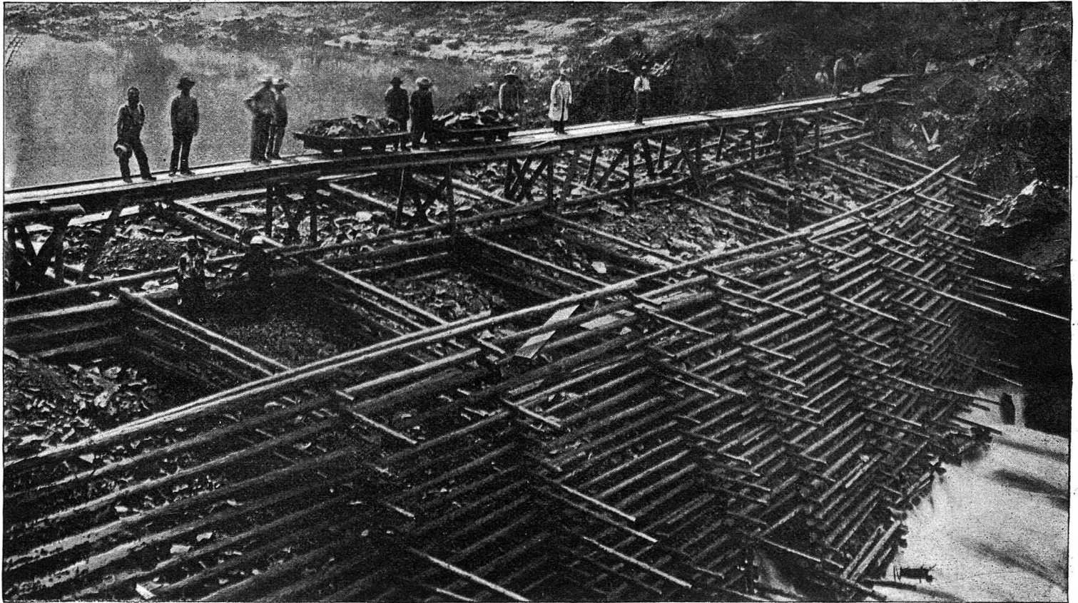
HEAD DAM, SHOWING PLAN OF CONSTRUCTION.
