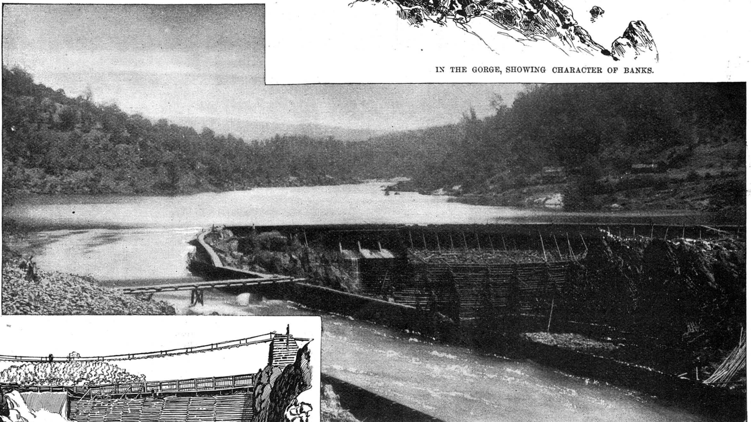
HEAD DAM, SHOWING WASTE-WAY CLOSED,
